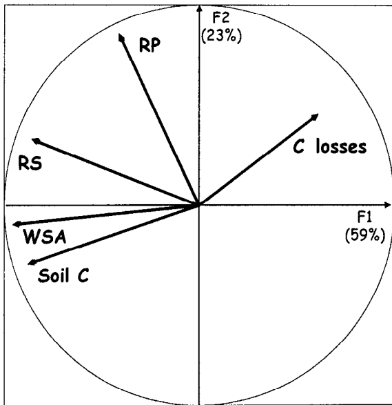
Figure 2a. F1-F2 correlation circle of variables (RP and RS are soil resistance to penetration and shear, respectively, and WSA water stable aggregates).
