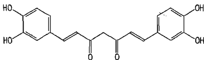
Figure 51 : Structure de la Dicafeoylméthane [69]
