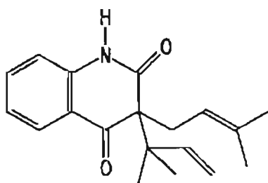
Figure 23 : Structure de la Buchapine [71]
