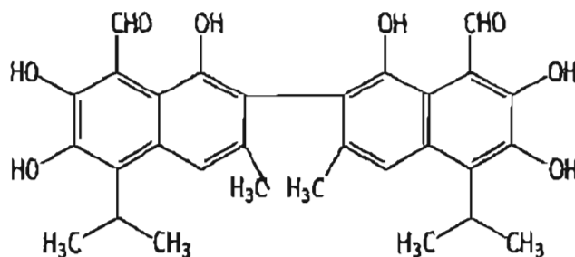
Figure 47 : Structure du gossypol [105]
