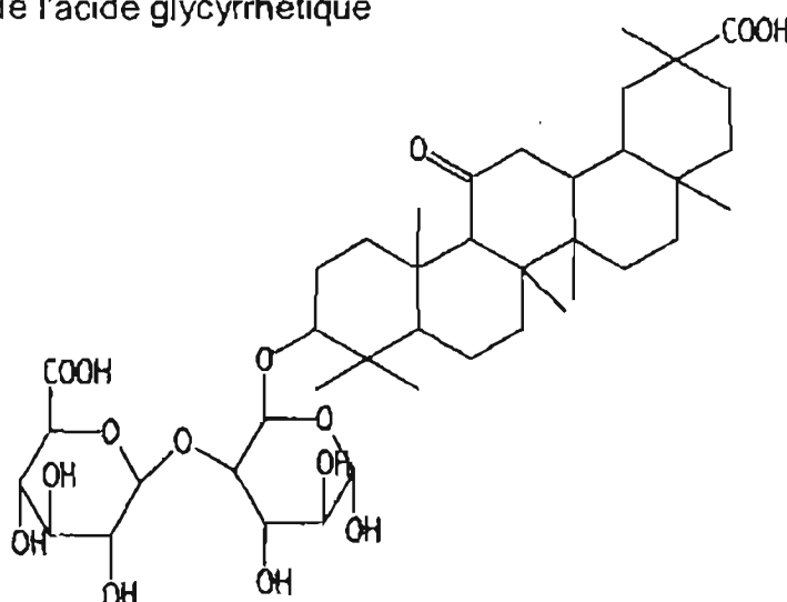
Figure 28 : Structure de la Glycyrrhizine [46]
